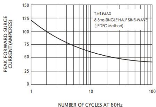
Figure 2: Forward Surge Current Curve
