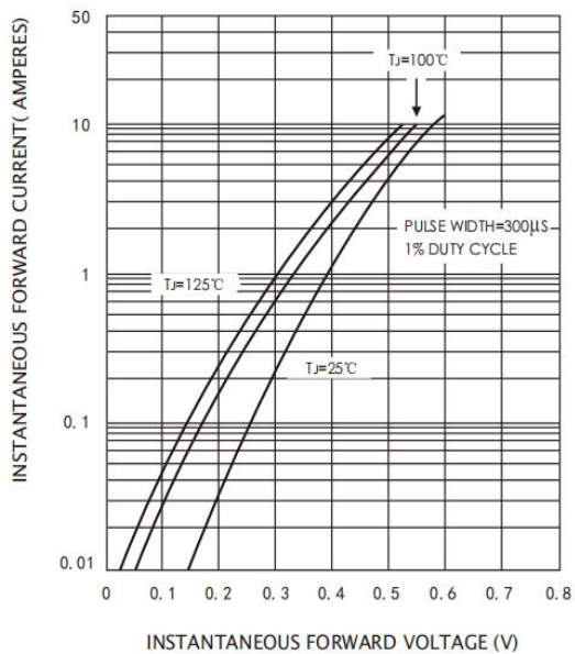
Figure 3: Forward Characteristics
