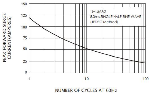
Figure 2: Forward Surge Current Curve
