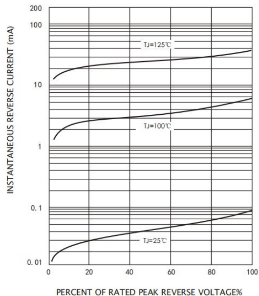
Figure 4: Reverse Characteristics
