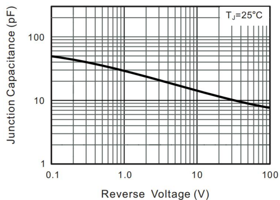
Figure 4: Junction Capacitance
